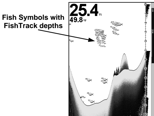
Sonar Page showing both the Fish I.D. symbol and FishTrack depth features turned on.
